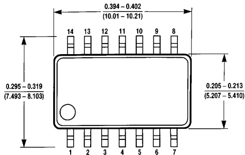
S.O. Package (M) Order Number DM64ALS32M or DM74ALS32M NS Package Number M14A
