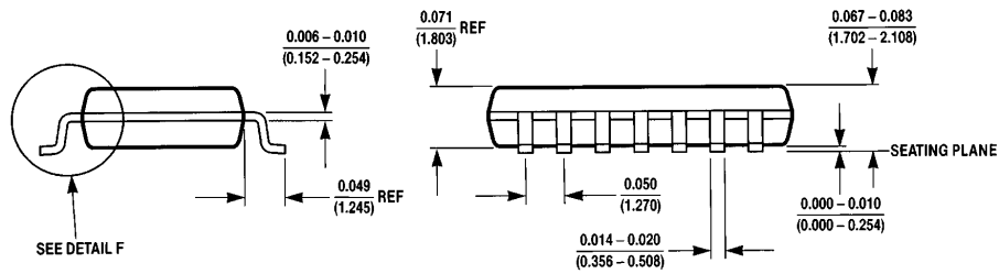
Small Outline Package (SJ) Order Number DM74ALS32SJ NS Package Number M14D
